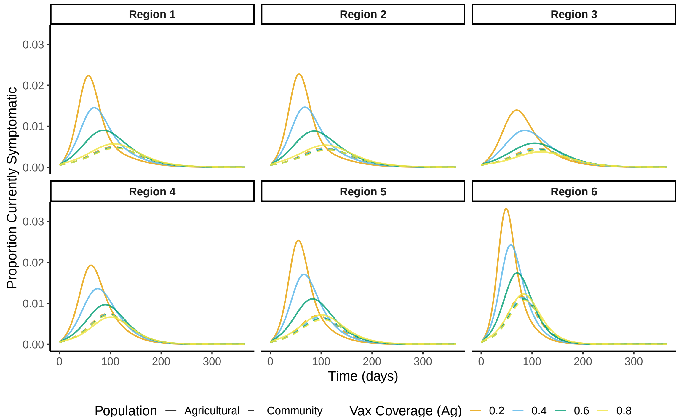
Symptomatic Cases by Region – Sensitivity to Vax Coverage (Ag)
