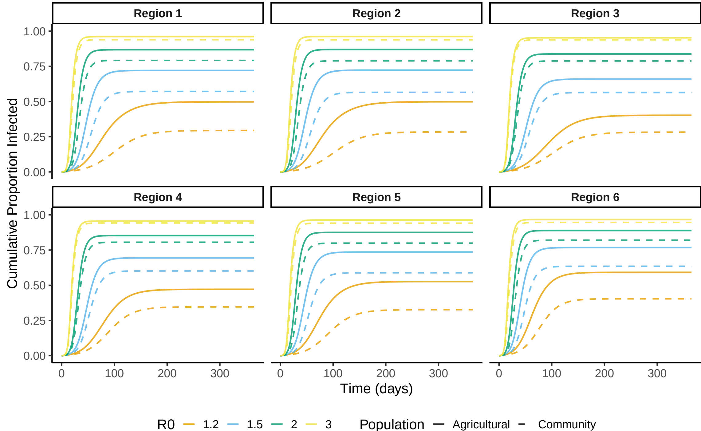
Cumulative Infections by Region – Sensitivity to R0
