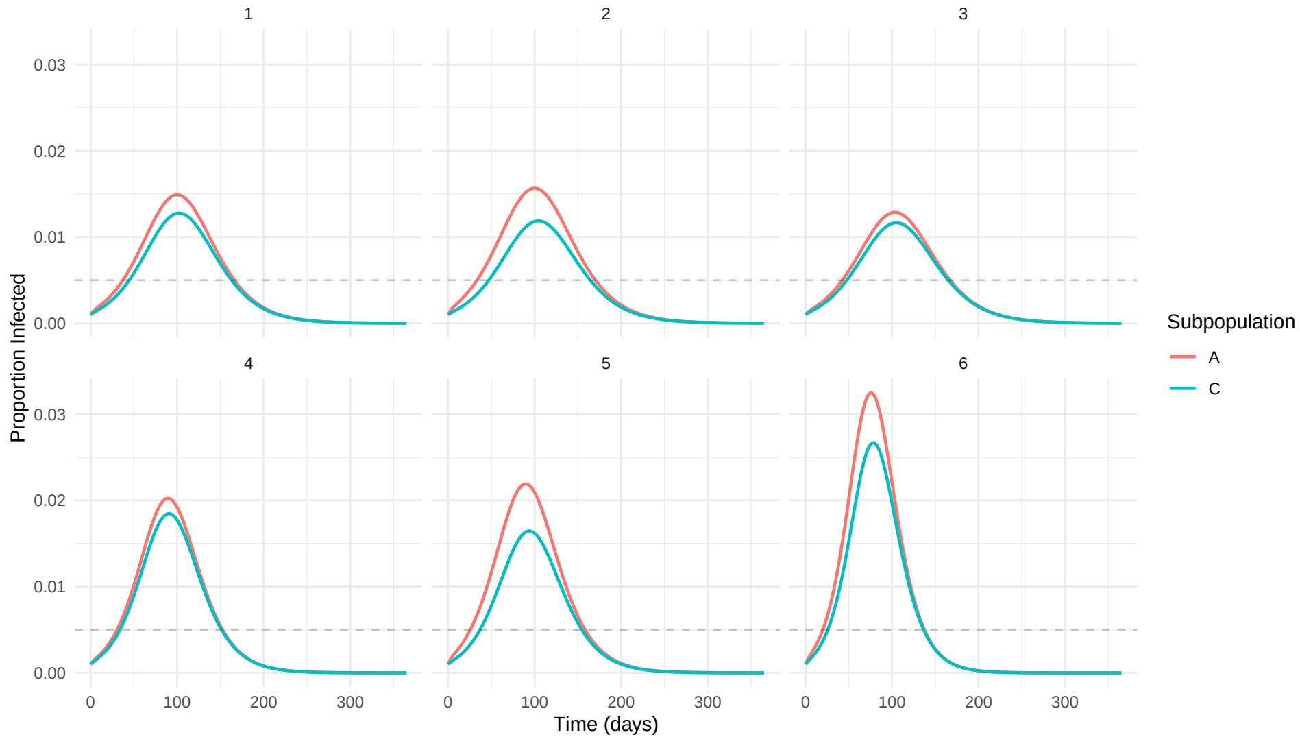
Infection curves: eps_0.7
