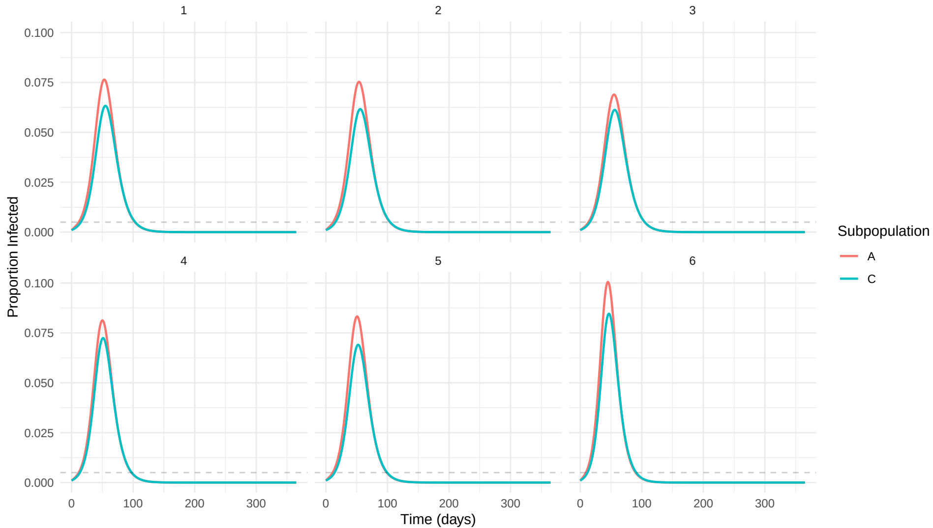
Infection curves: eps_1
