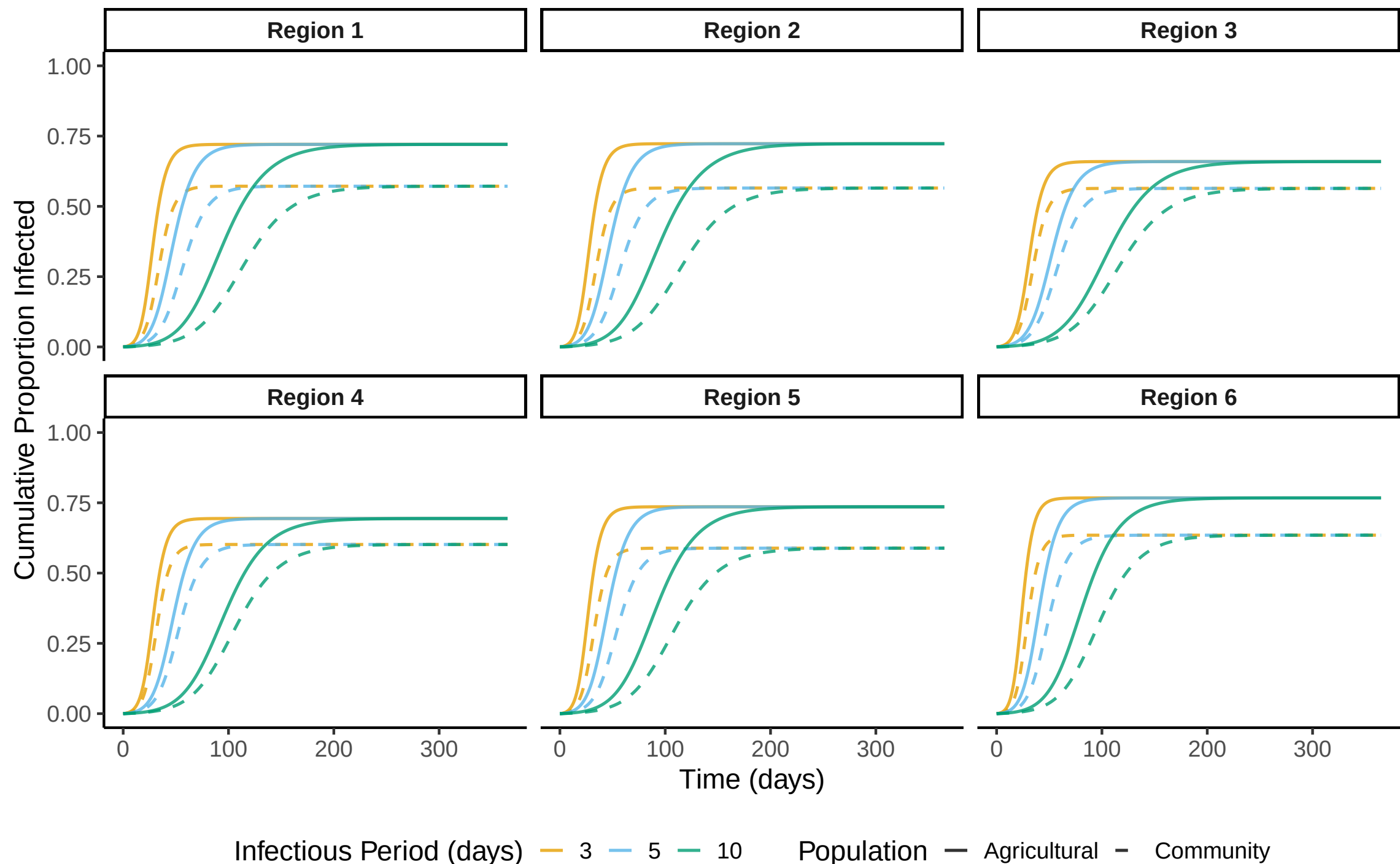
Cumulative Infections by Region – Sensitivity to Infectious Period (days)
