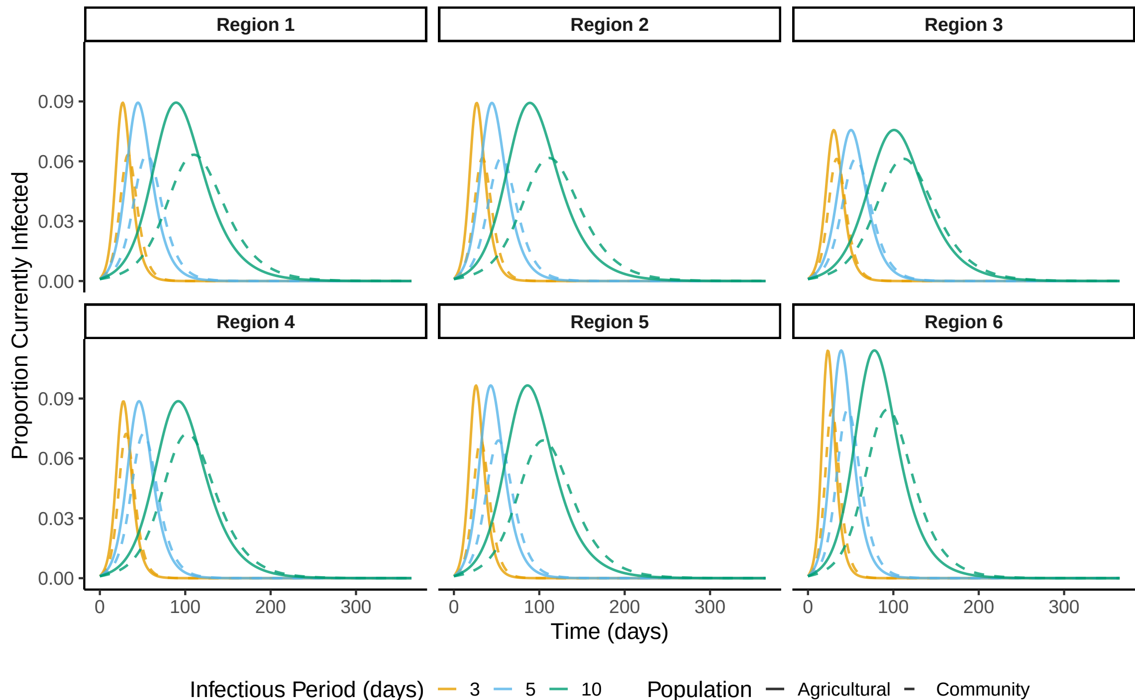
Epidemic Curves by Region – Sensitivity to Infectious Period (days)
