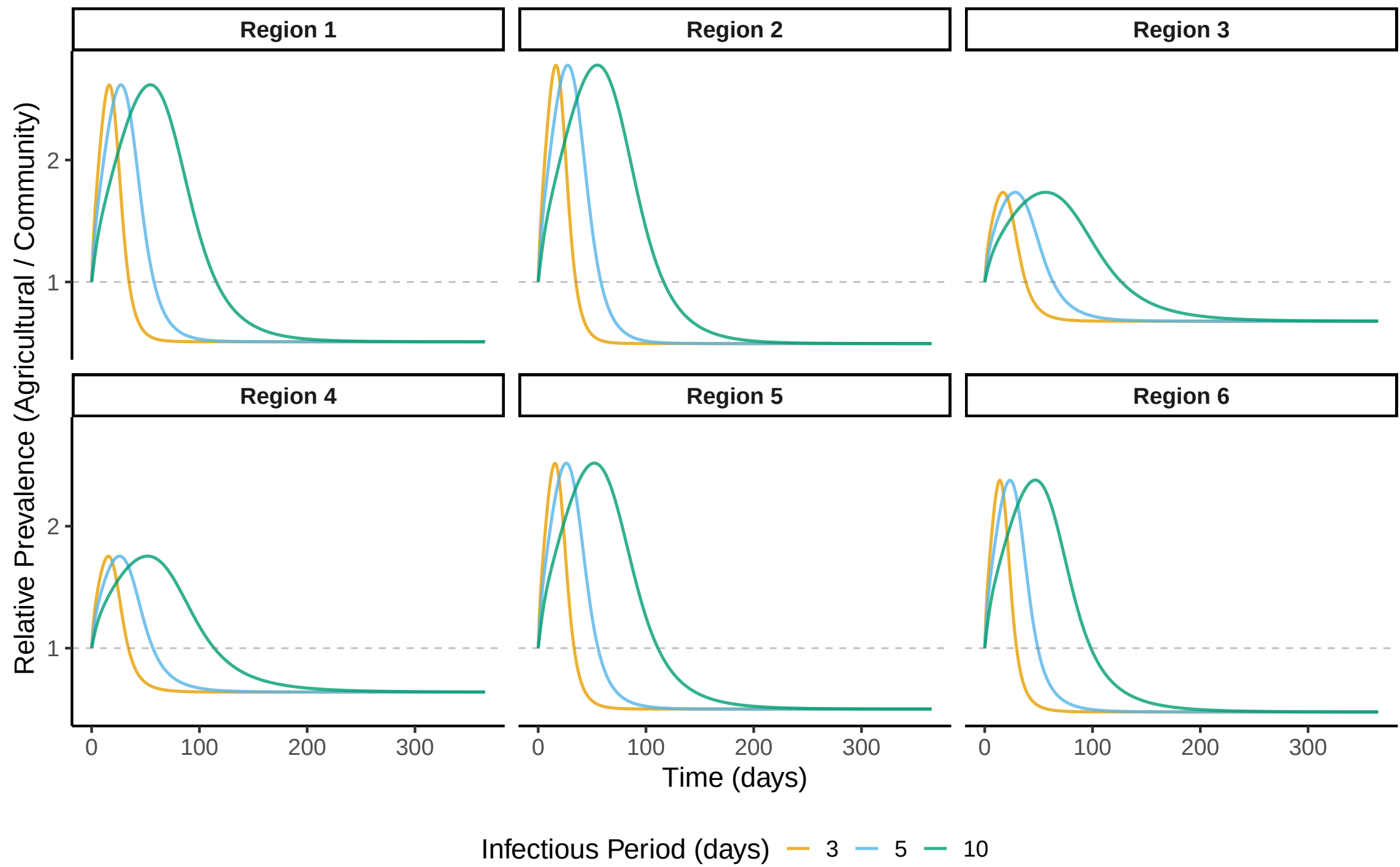
Relative Prevalence by Region – Sensitivity to Infectious Period (days)
