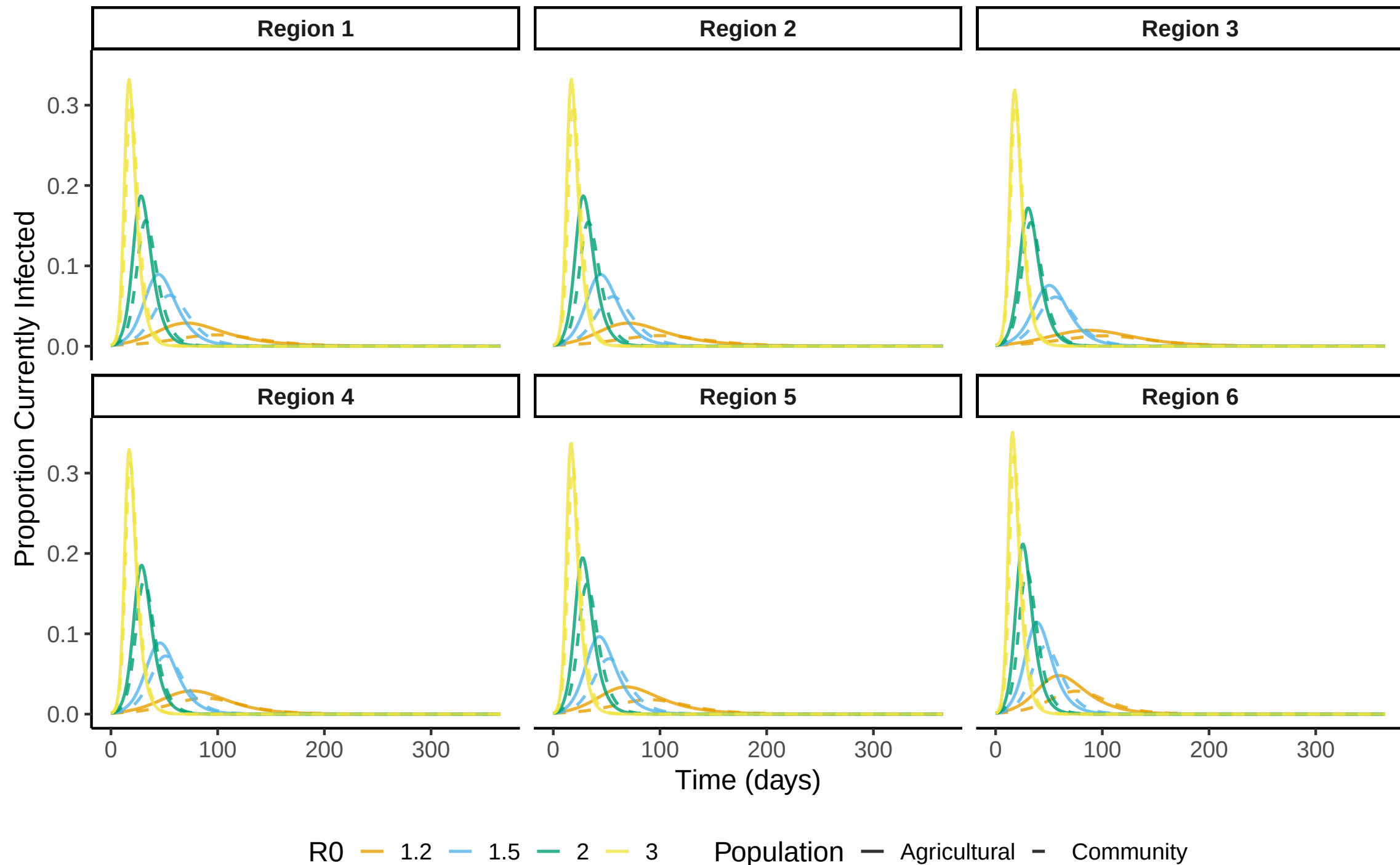
Epidemic Curves by Region – Sensitivity to R0
