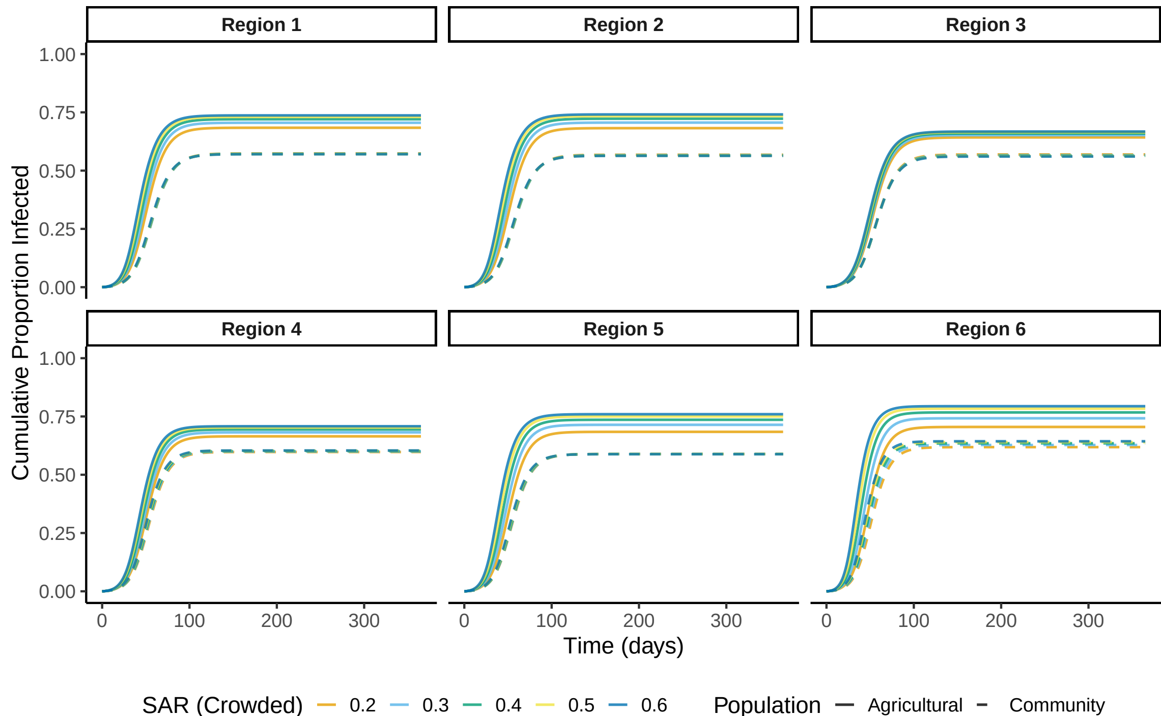
Cumulative Infections by Region – Sensitivity to SAR (Crowded)
