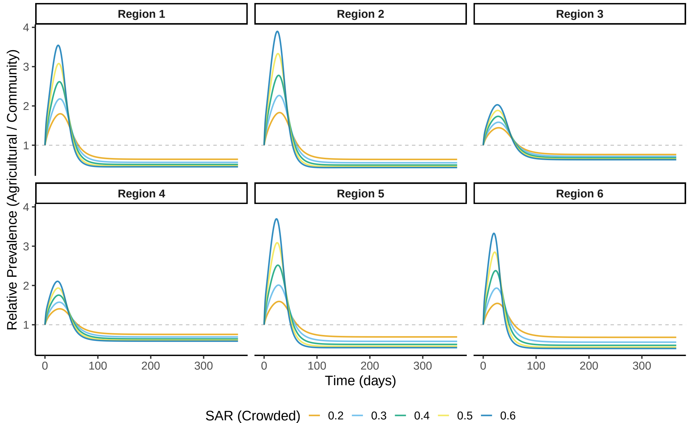
Relative Prevalence by Region – Sensitivity to SAR (Crowded)
