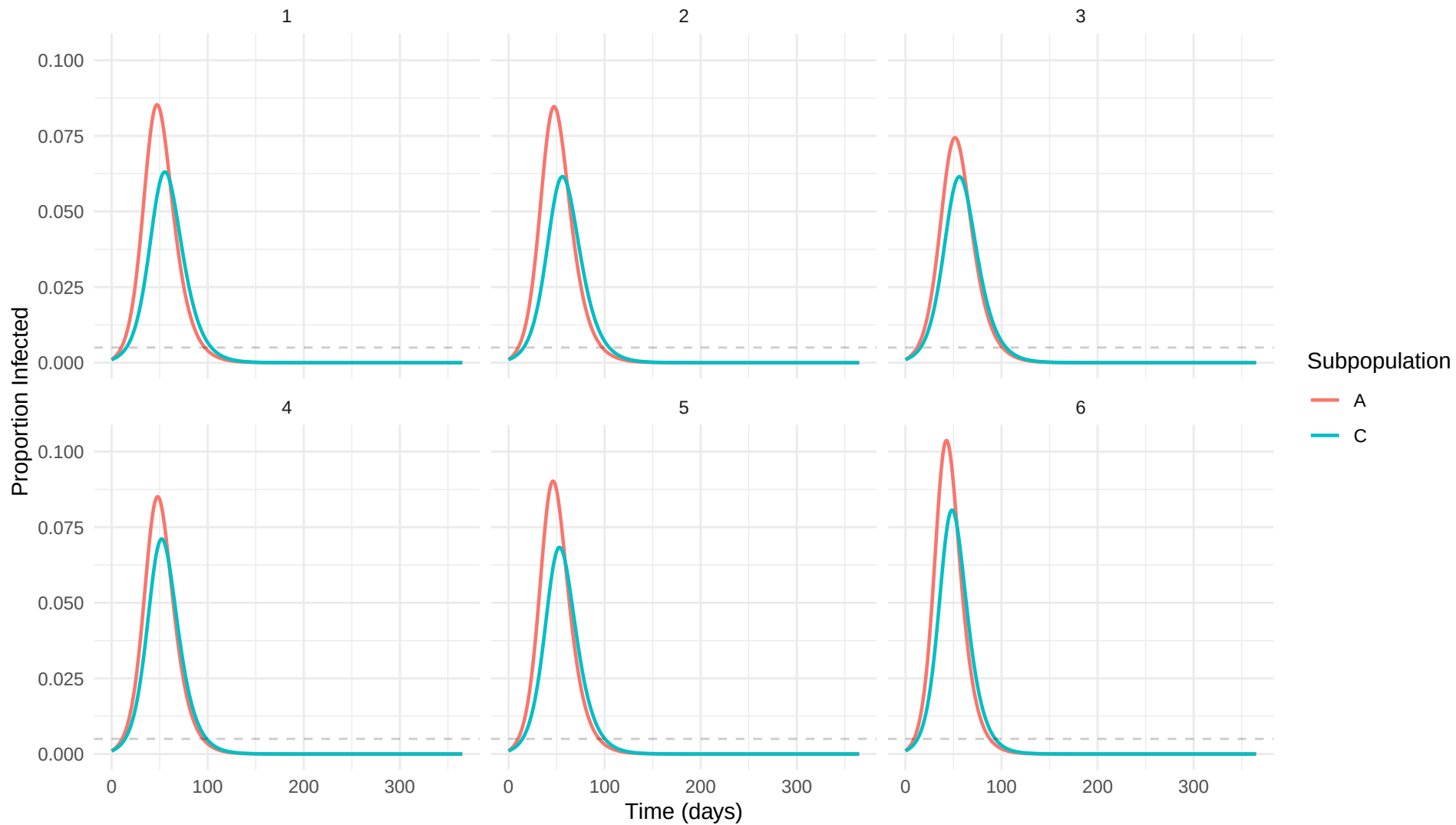
Infection curves: sar_0.3
