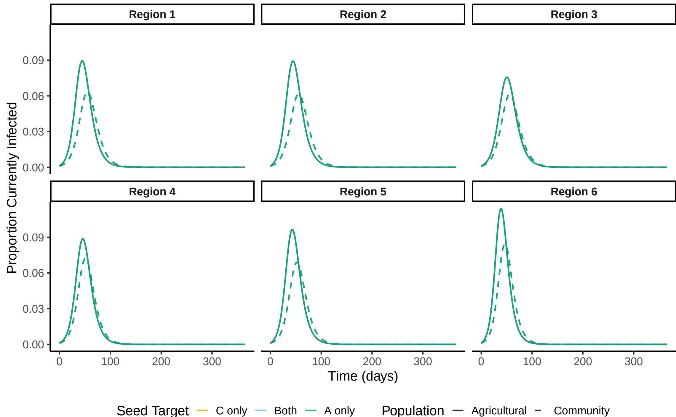
Epidemic Curves by Region – Sensitivity to Seed Target
