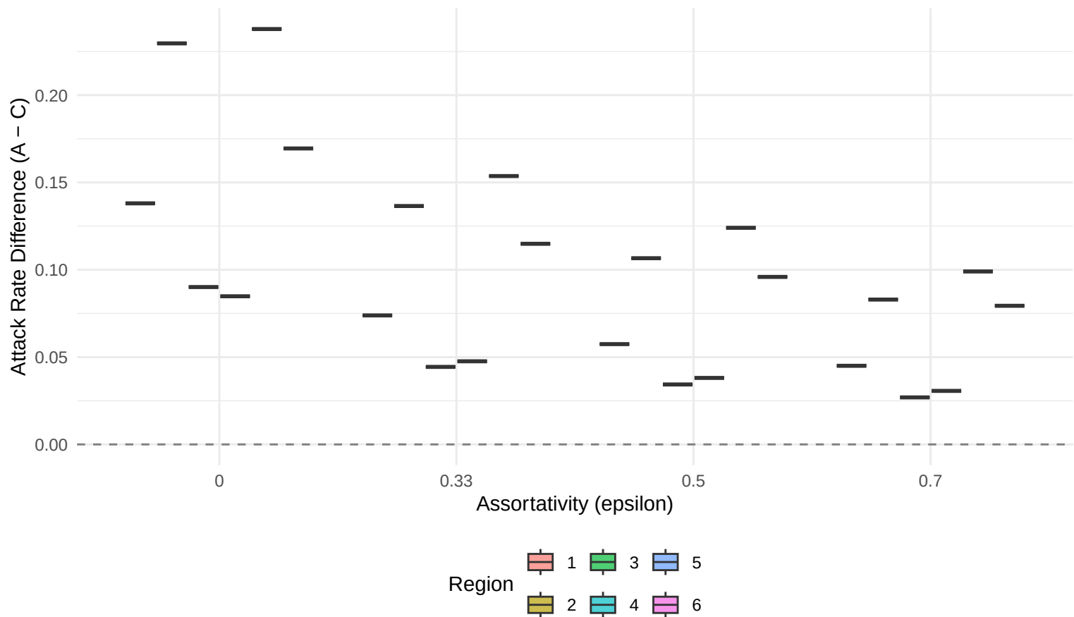
Sensitivity to Assortativity (epsilon)
