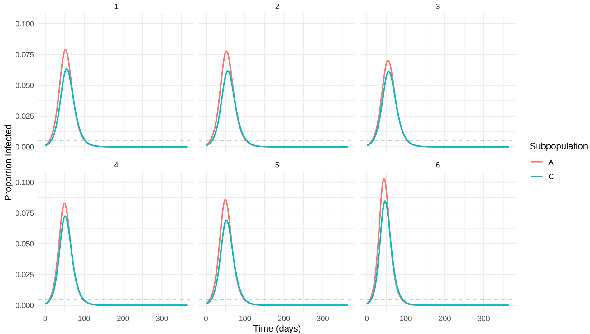
Infection curves: \text{eps\_}0.75
