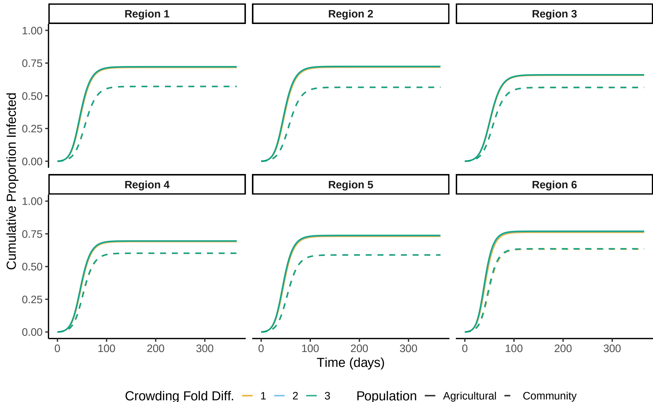
Cumulative Infections by Region – Sensitivity to Crowding Fold Diff.
