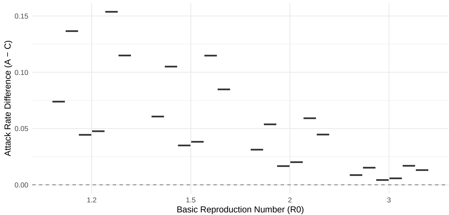
Sensitivity to Basic Reproduction Number (R0)
