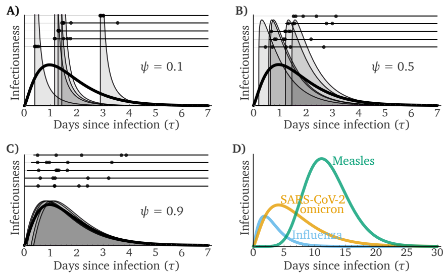
Figure 1 | The individual infectiousness kernel and the burstiness parameter \psi .
