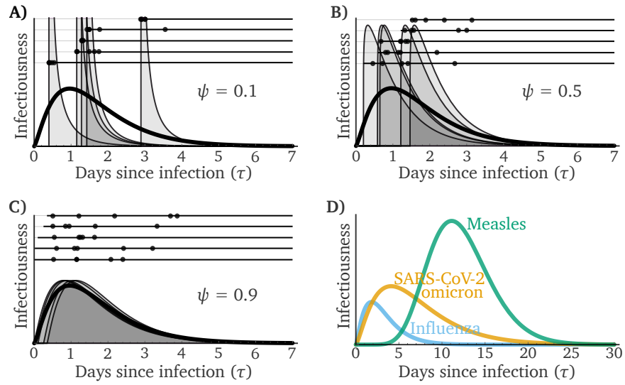
Figure 1 | The individual infectiousness kernel and the burstiness parameter \psi . Caption of the first figure goes here. What does the font look like?
