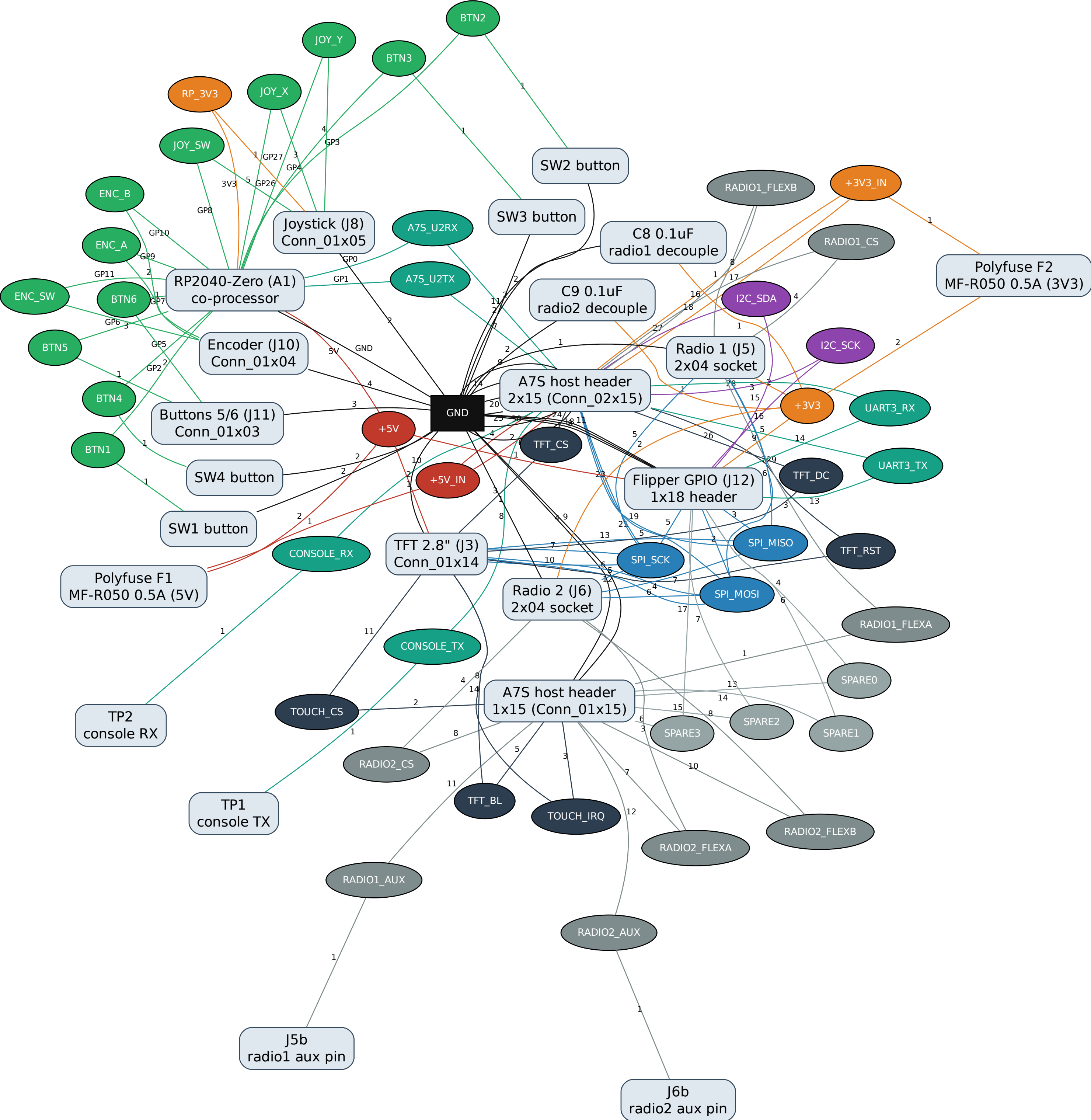
A7S Cyberdeck Backplane — connectivity diagram (generated from a7s_backplane_skidl.py — the schematic source of truth)
