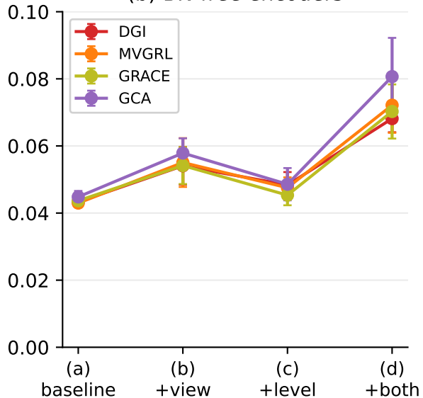
(b) BN-free encoders
