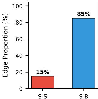
Transaction Graph
