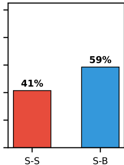
Behavioral k-NN
