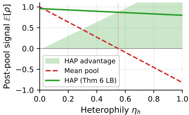
(b) Mean vs HAP ( k = 10, \varepsilon = 0.2 )
