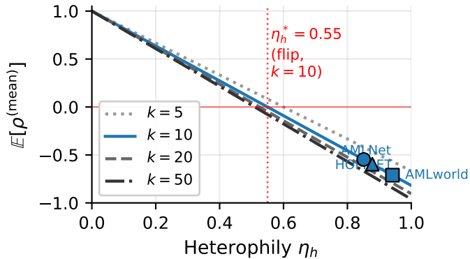
(a) Mean-pool signal flip (Thm~5)
