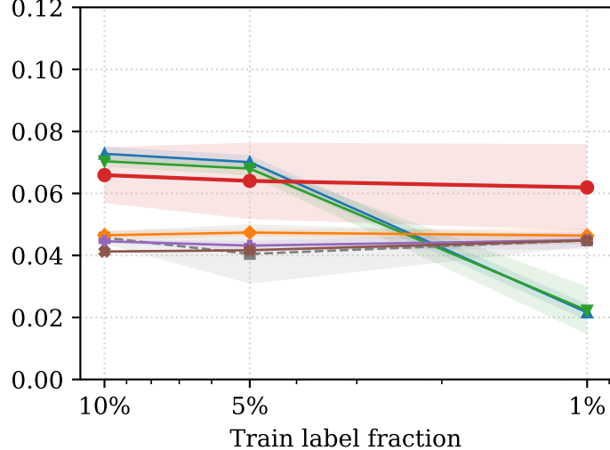
AMLworld ( \rho = 1.23\% )
