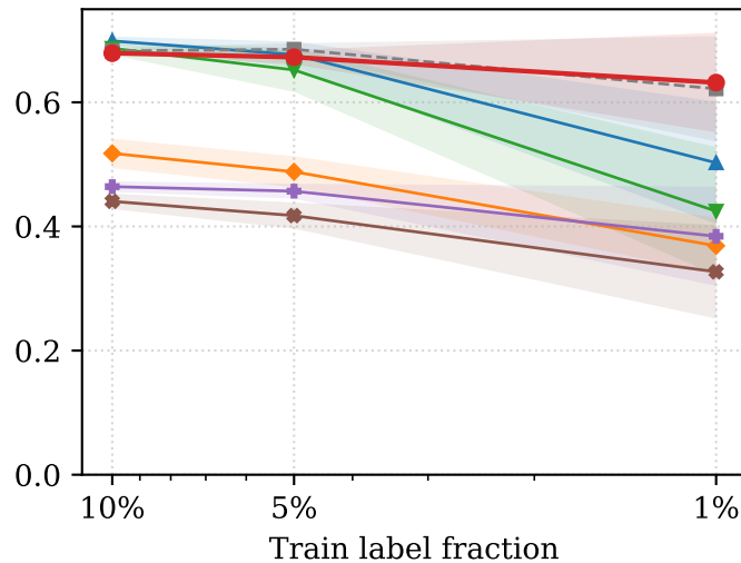
AMLNet ( \rho = 13.52\% )
