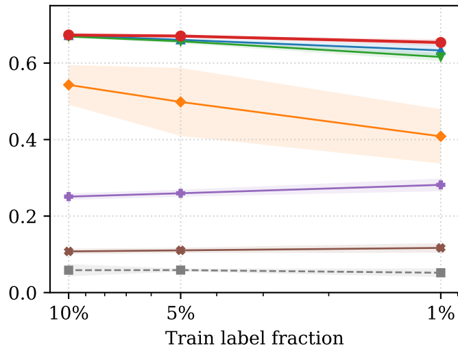
HOFINET ( \rho = 2.13\% )
