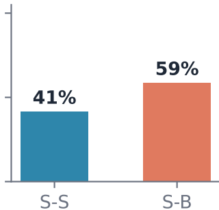
Behavioral k-NN
