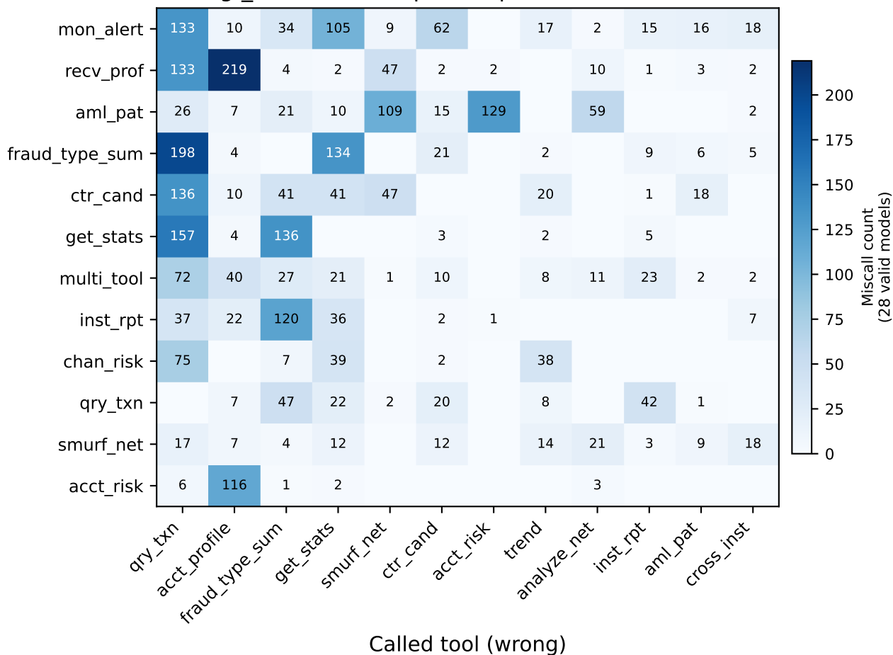
Tool confusion matrix: expected vs. ~called tool (wrong\_func errors, top-12 expected tools, 28 models)
