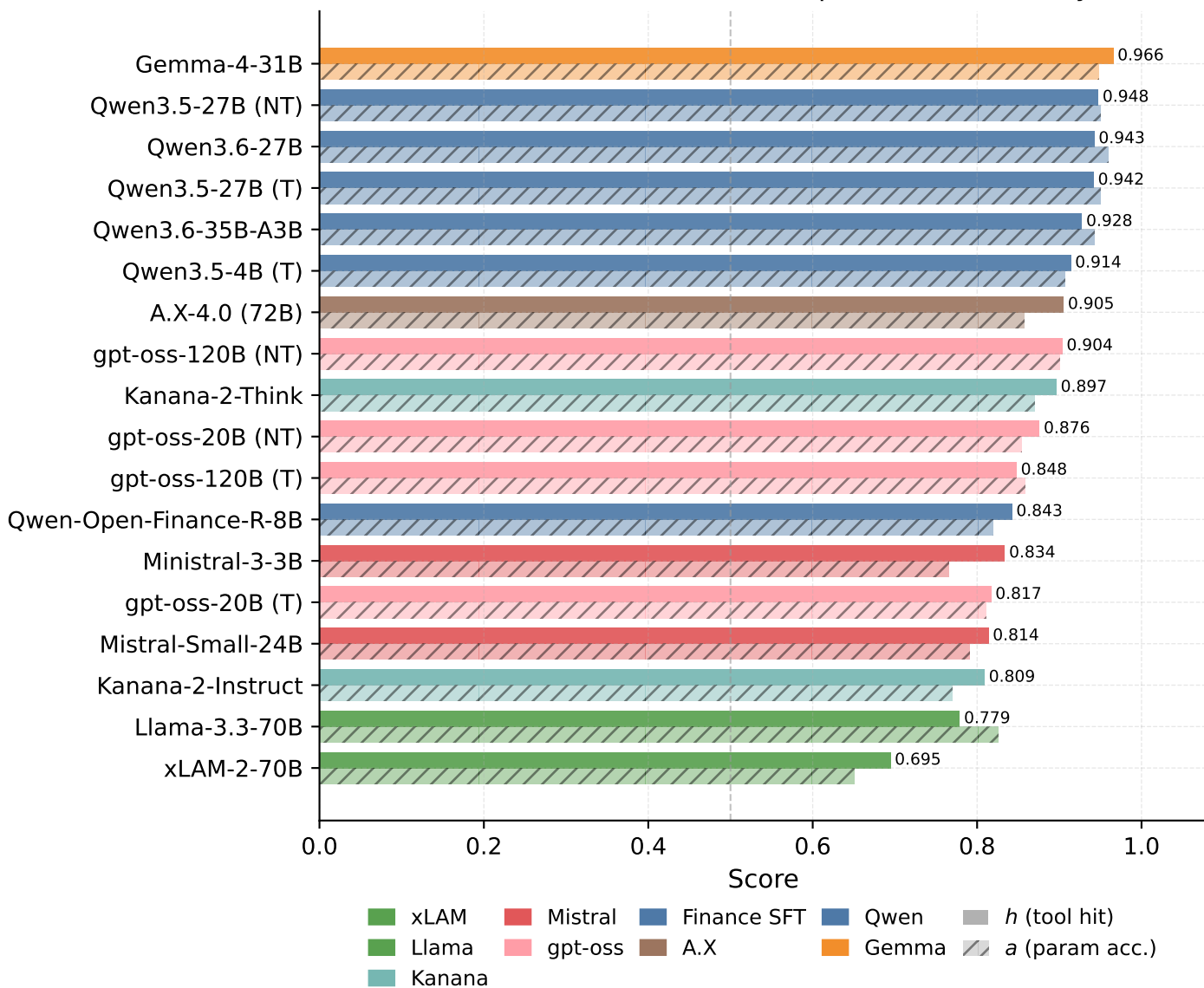
Tool hit h and parameter accuracy a , 18 of 28 configurations (Korean tool schema, Korean questions; sorted by h )
