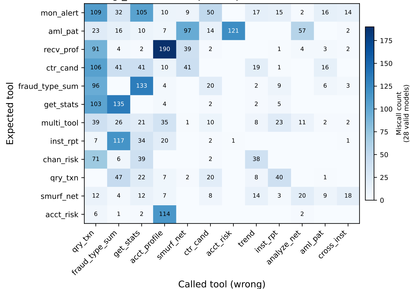
Tool confusion matrix: expected vs. ~called tool (wrong\_func errors, top-12 expected tools, 28 models)
