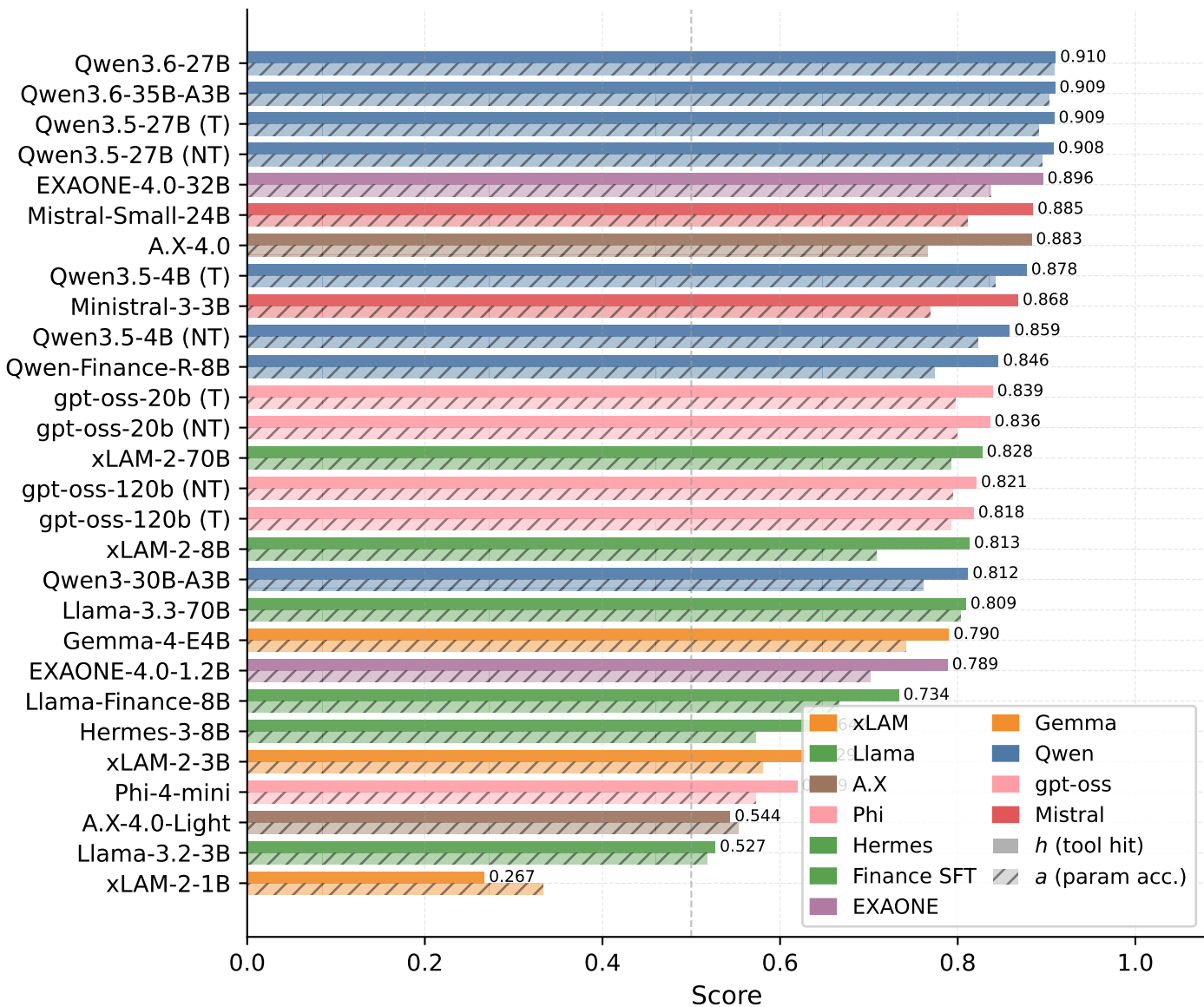
Tool hit h and parameter accuracy a across 28 valid models (Korean prompts, thinking off; sorted by h )
