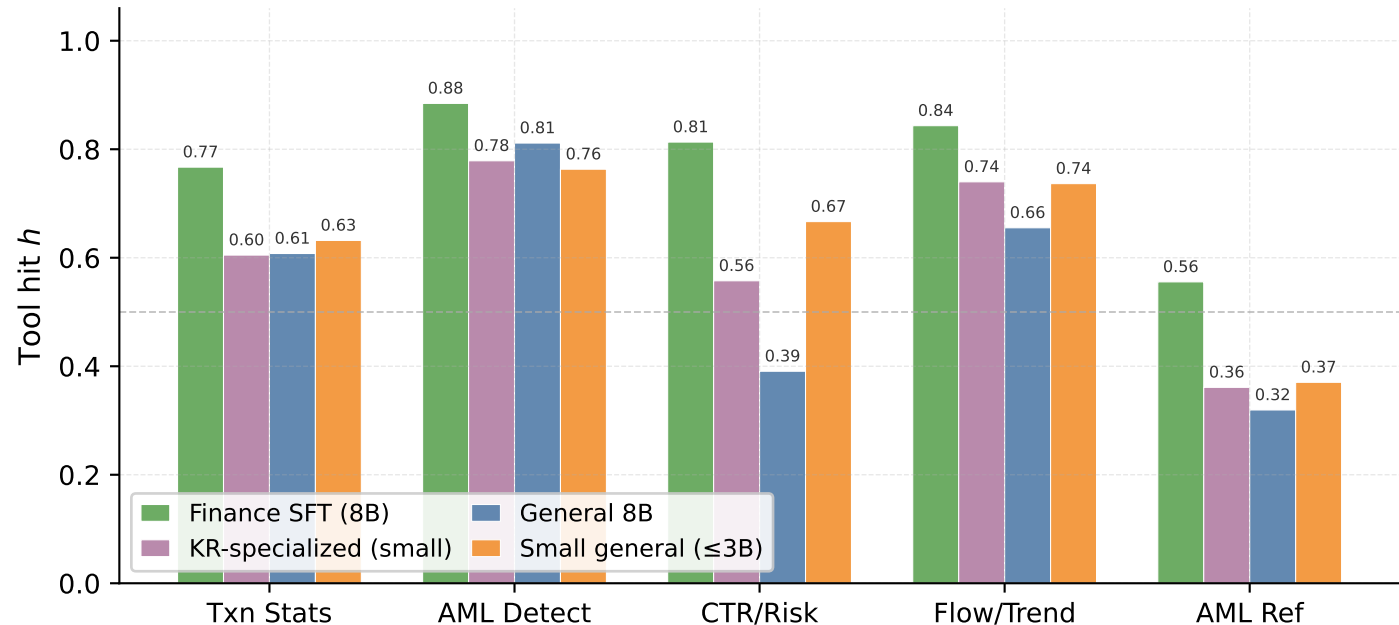
Subdomain tool hit h by model group (Finance SFT, KR-specialized, General 8B, Small general)
