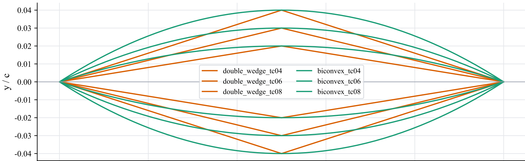
Digitized NACA RM A53B02 sections
