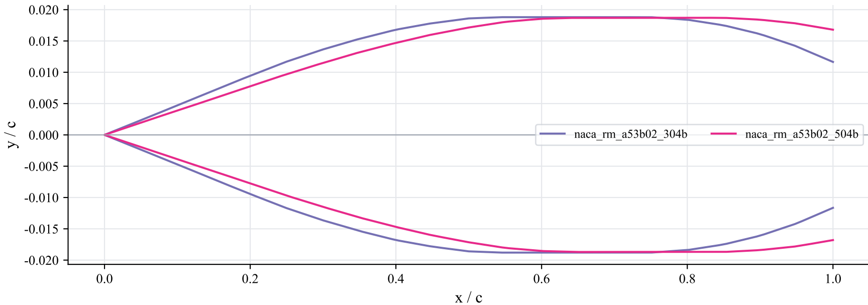
Digitized NACA RM A53B02 sections
