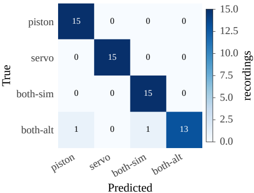
(a) Random forest - 97%
