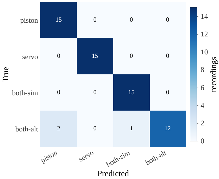
(b) LDA - 95%
