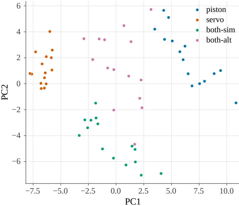
(a) PCA (unsupervised) - 55% variance
