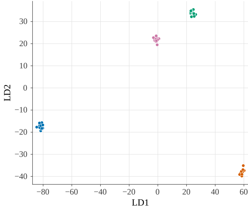
(b) LDA (supervised)
