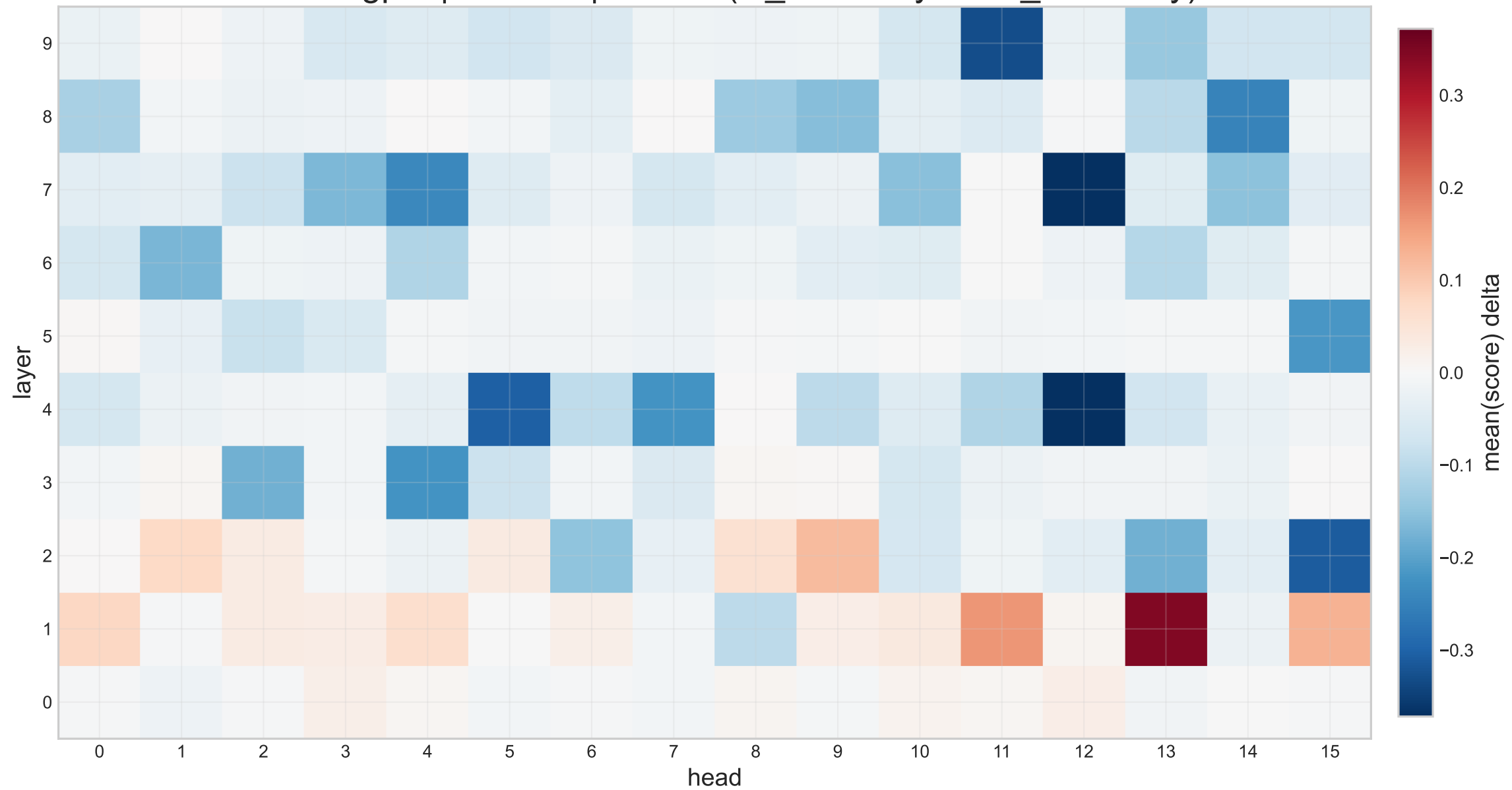
toksuite/gpt2 | chinese | \Delta score (in_boundary – out_boundary)
