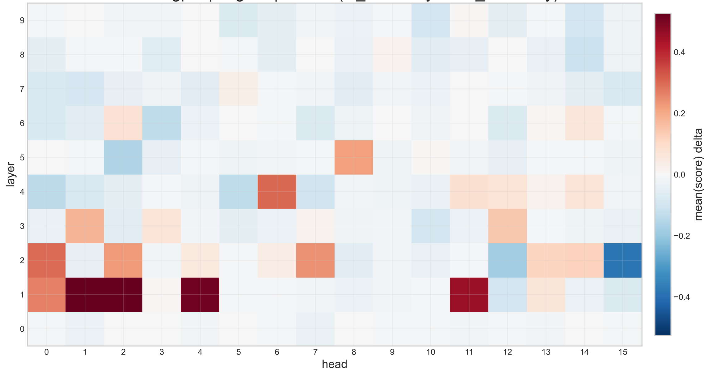
toksuite/gpt2 | english | \Delta score (in_boundary - out_boundary)
