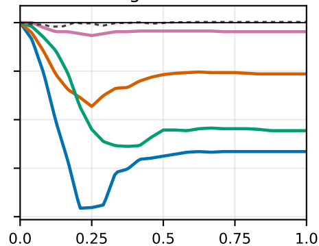
5% targeted – clean
