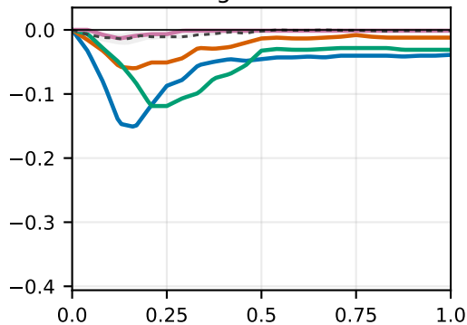
1% targeted – clean
