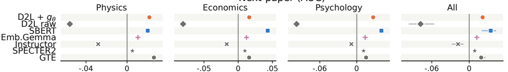
Topic (macro-F1)
