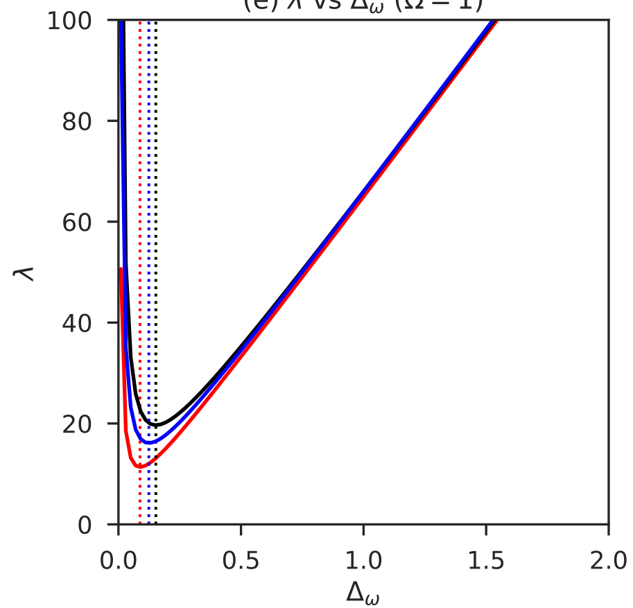
(e) \lambda vs \Delta_\omega ( \Omega = 1 )
