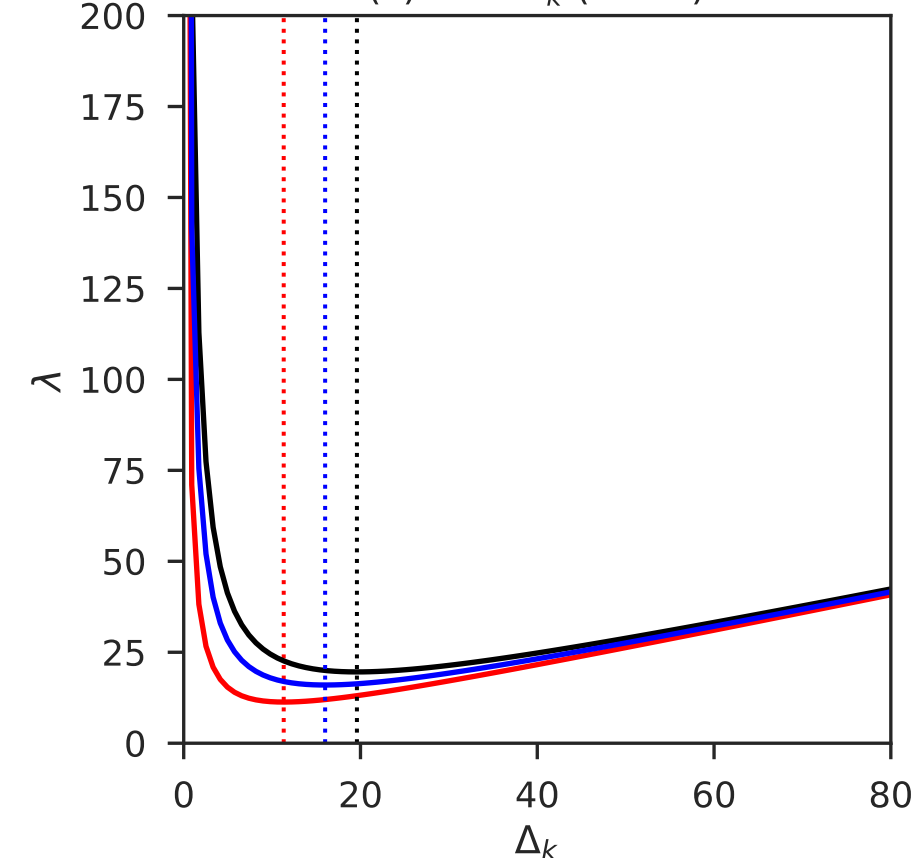
(c) \lambda vs \Delta_k ( \Omega = 1 )
