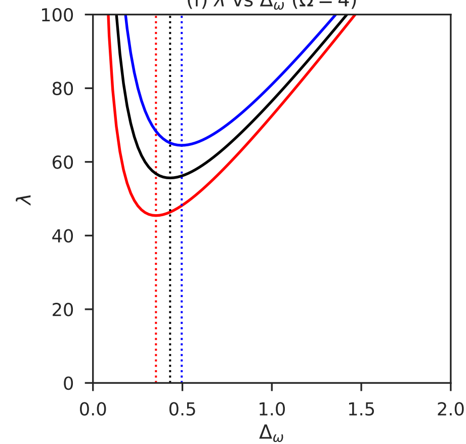
(f) \lambda vs \Delta_\omega ( \Omega = 4 )
