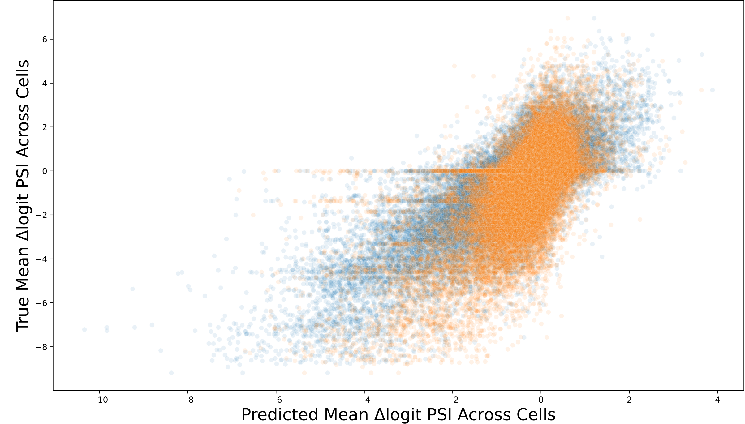
Retrained MMSplice \Delta logit PSI vs Pretrained on Train Set (Retrained r=0.778 , Baseline r = 0.658 )
