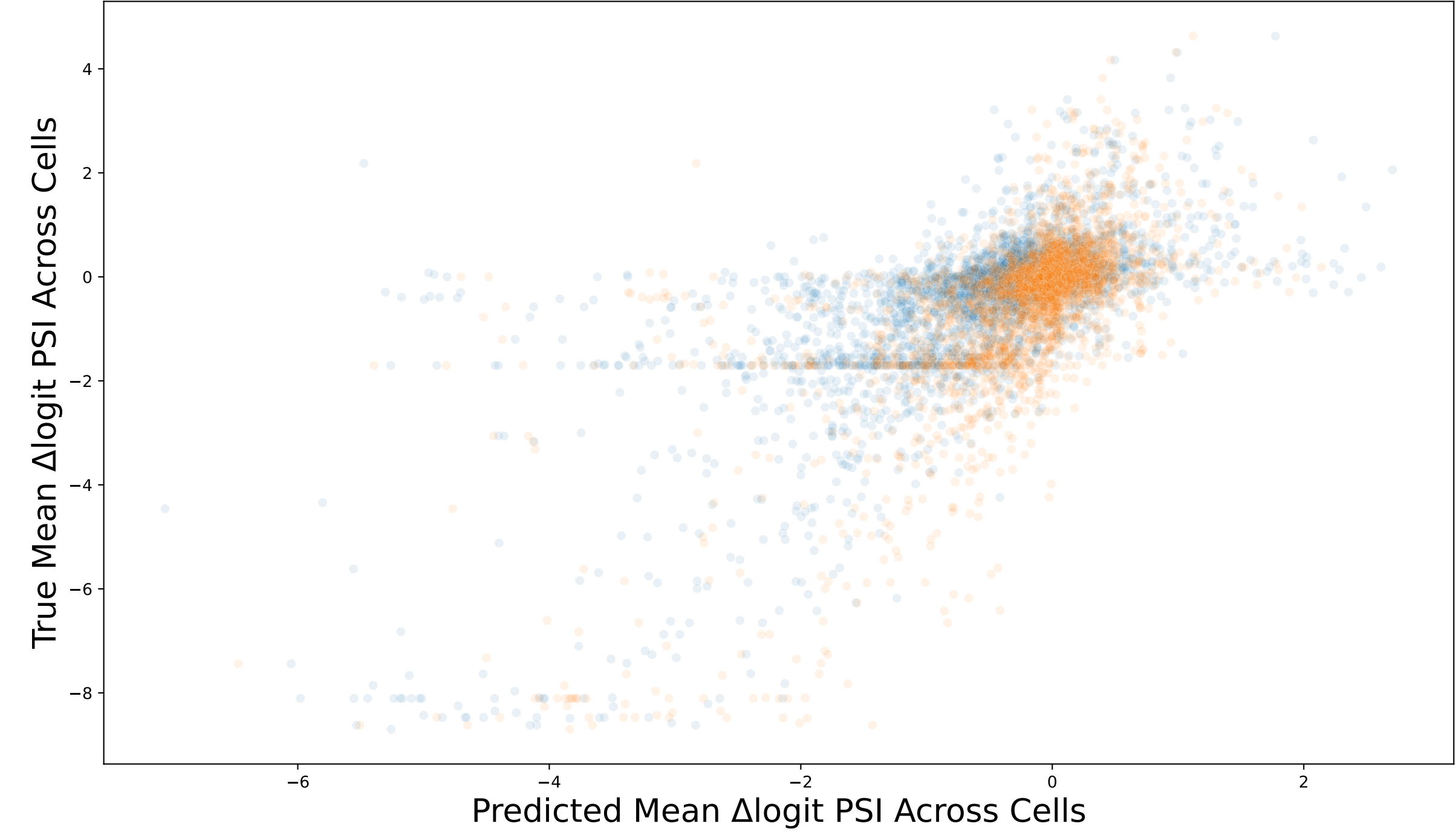
Retrained MMSplice \Delta logit PSI vs Pretrained on Validation Set (Retrained r=0.695 , Baseline r = 0.676 )
