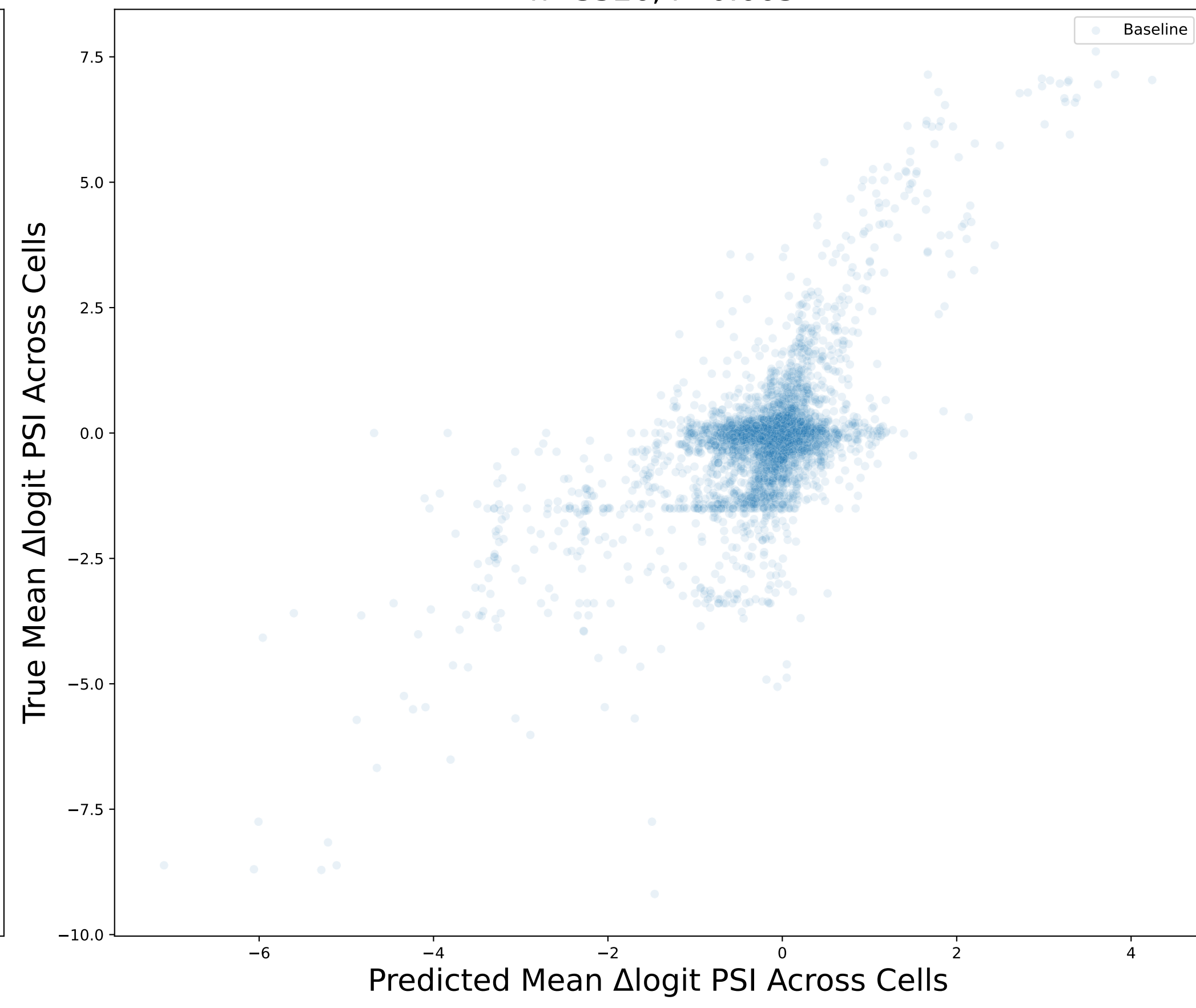
Test Set Baseline n=3526, r=0.663
