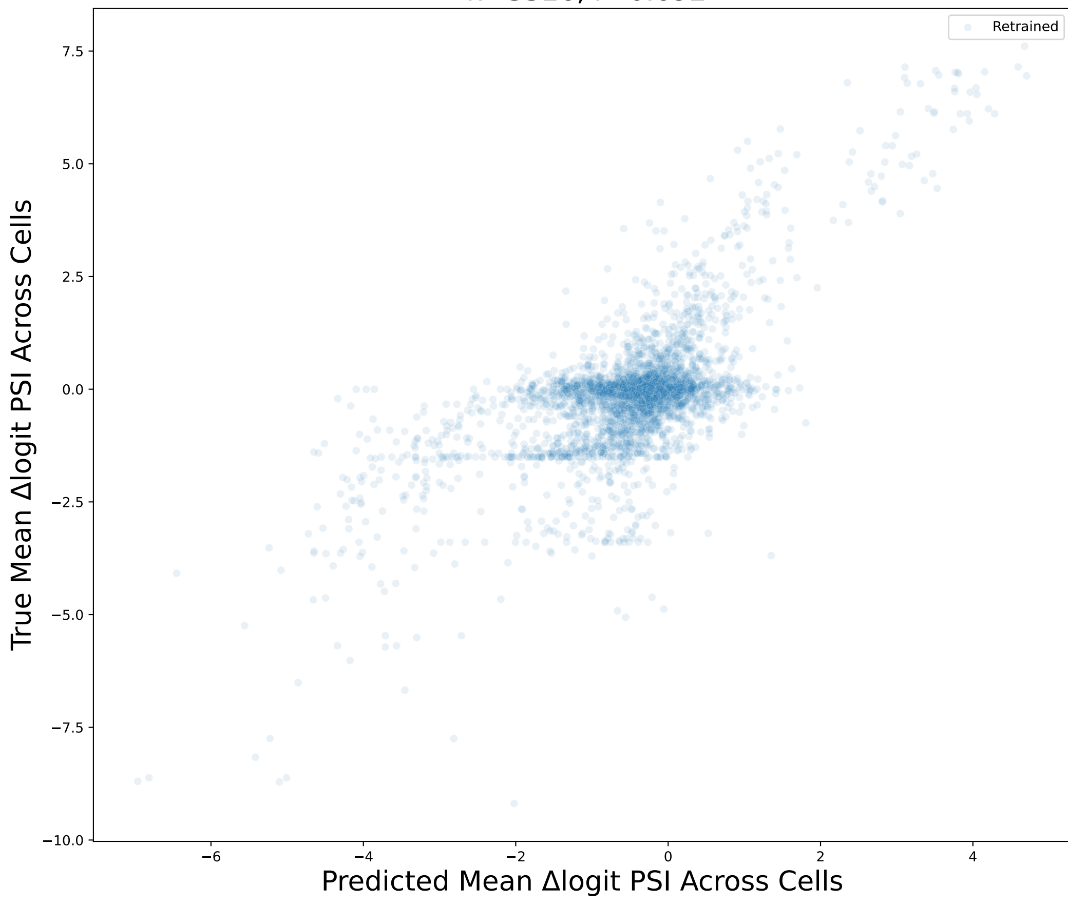
Test Set Retrained n=3526, r=0.692
