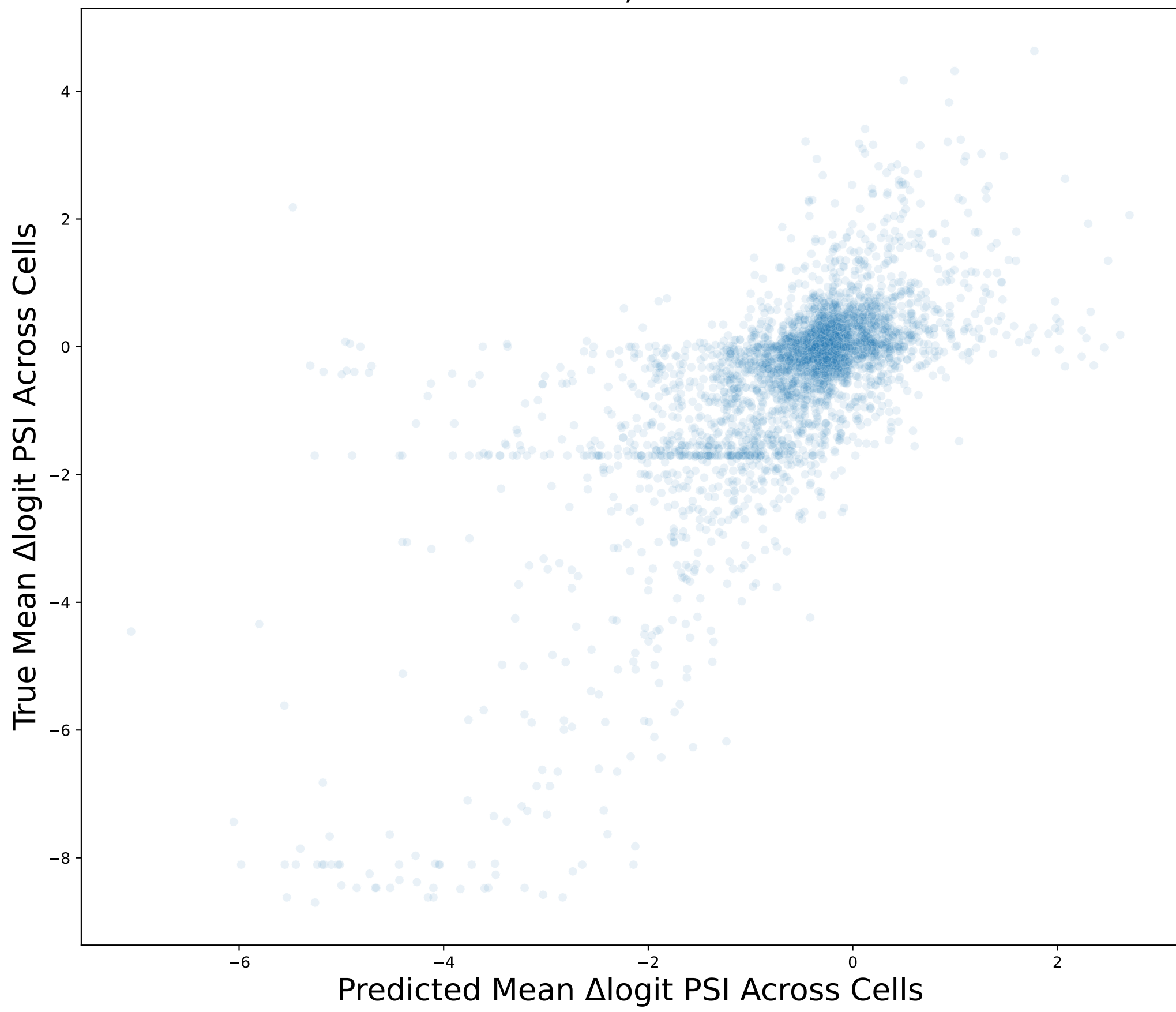
Test Set Retrained n=3526, r=0.692
