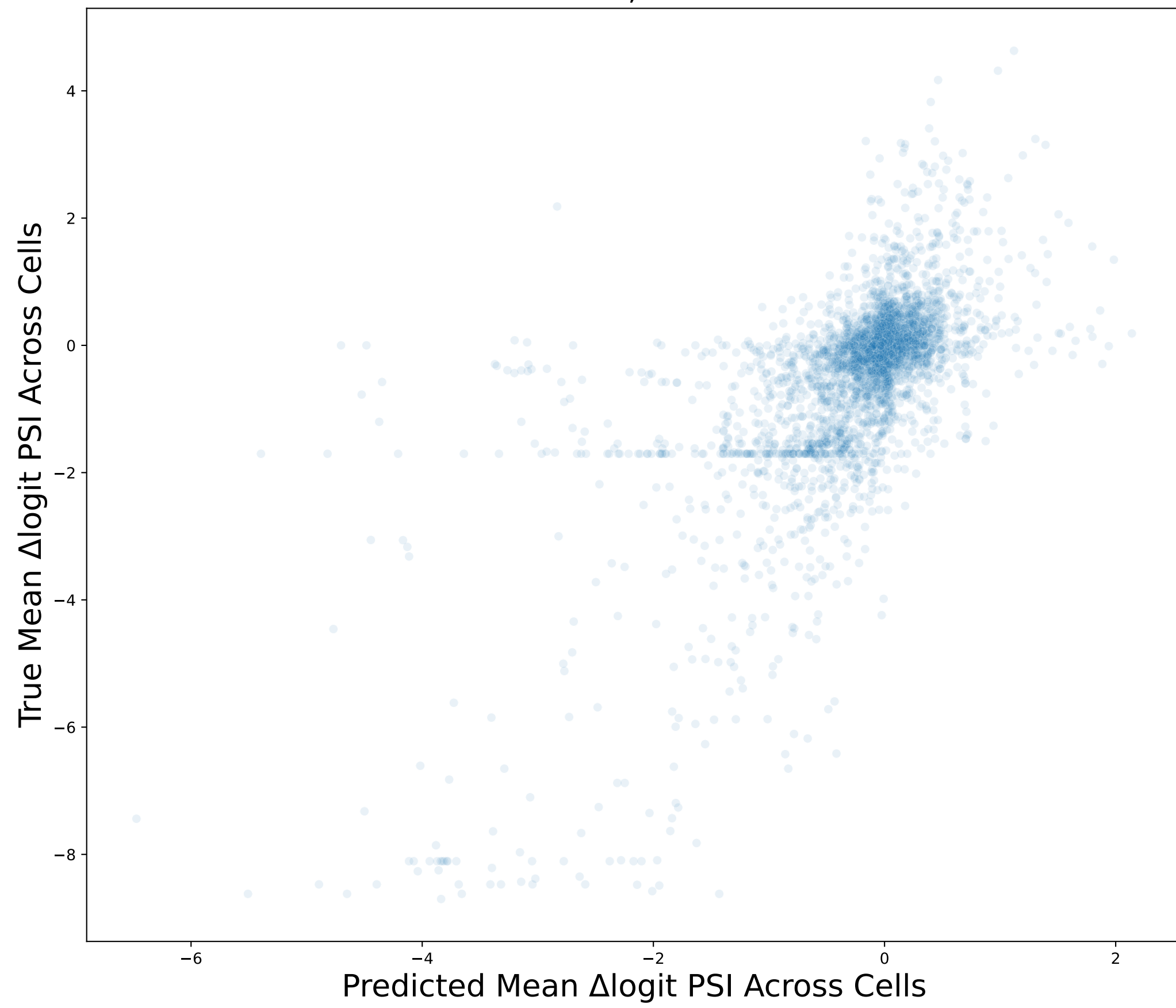
Test Set Baseline n=3526, r=0.663
