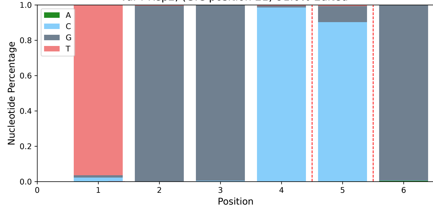
Var4 Rep2, (G:C position 21) 91.0% Edited
