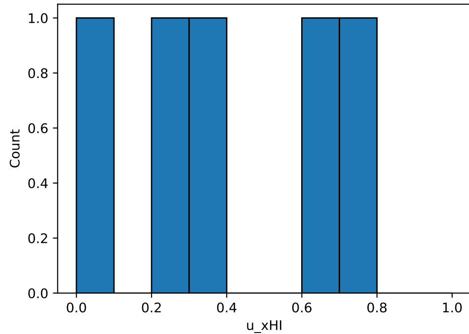
PIT Histogram for xHI
