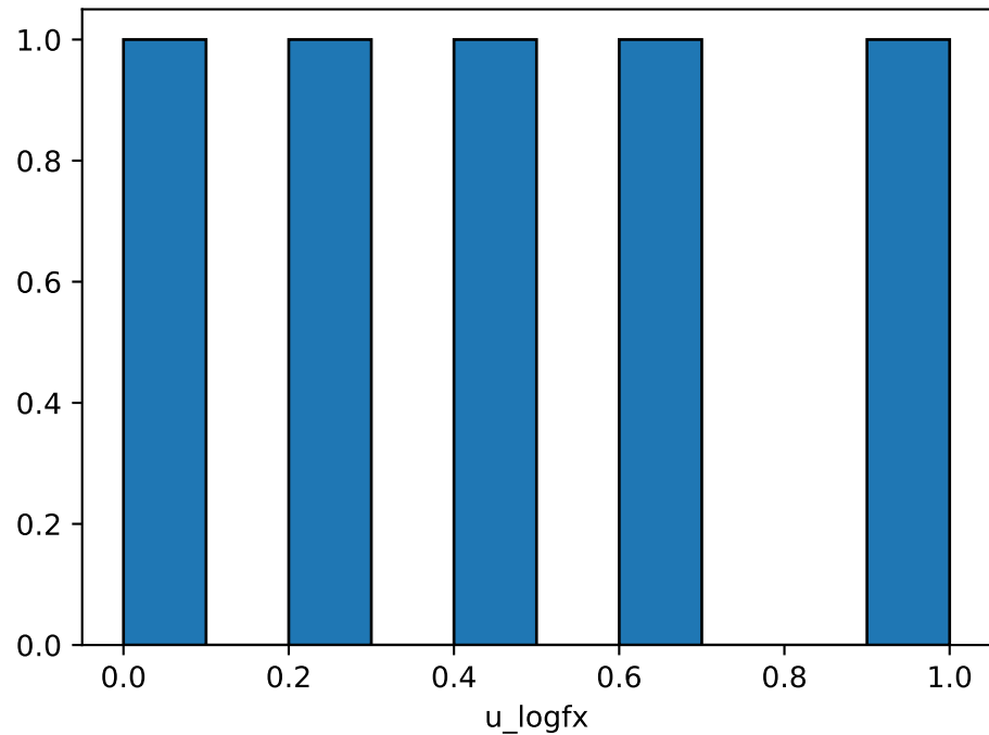
PIT Histogram for log fX
