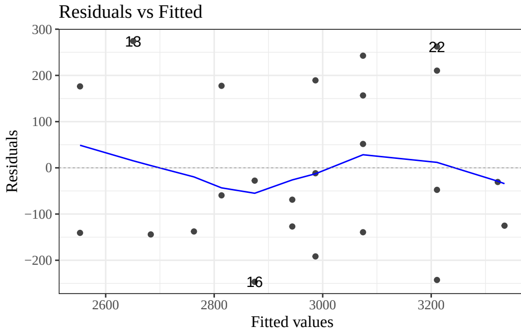
Figure 25: birthweight model (Equation 2): residuals versus fitted values
