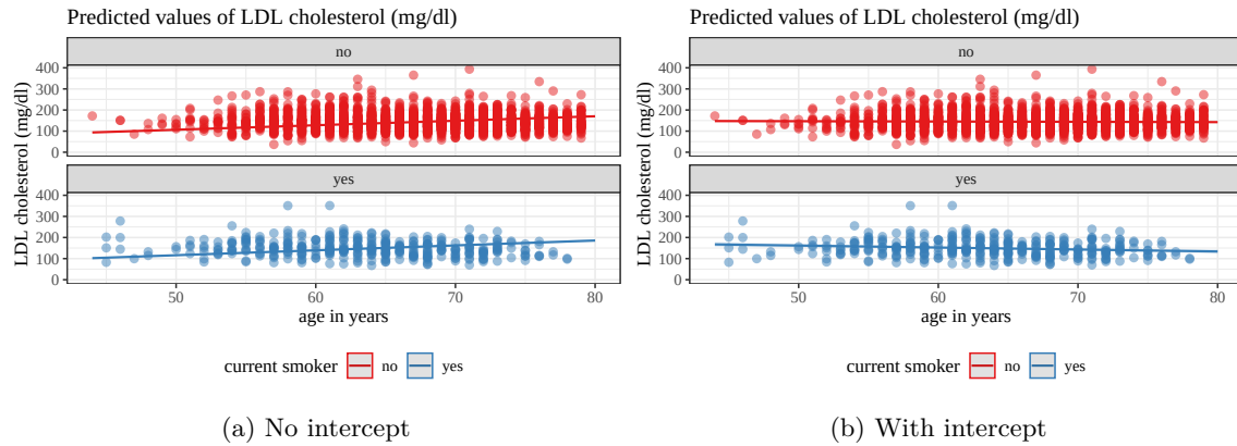
Figure 15: hers data models with and without intercepts
