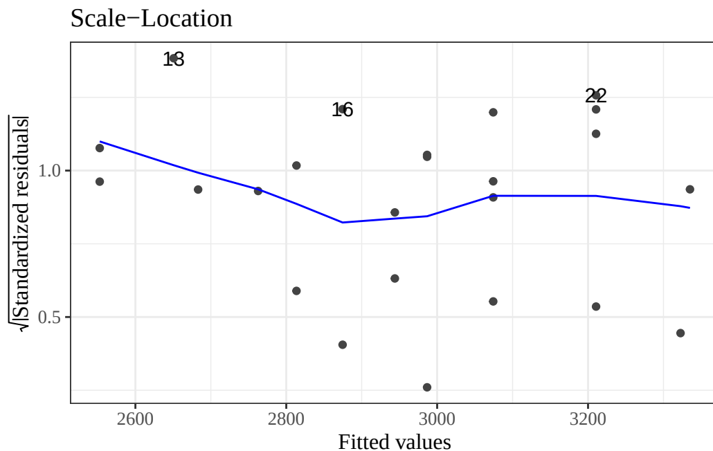
Figure 33: Scale-location plot of birthweight data
