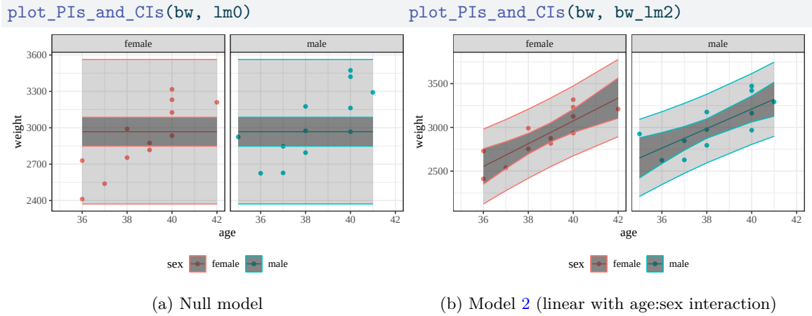
Figure 12: Null model and model 2 for birthweight data, with 95% confidence and prediction intervals.
