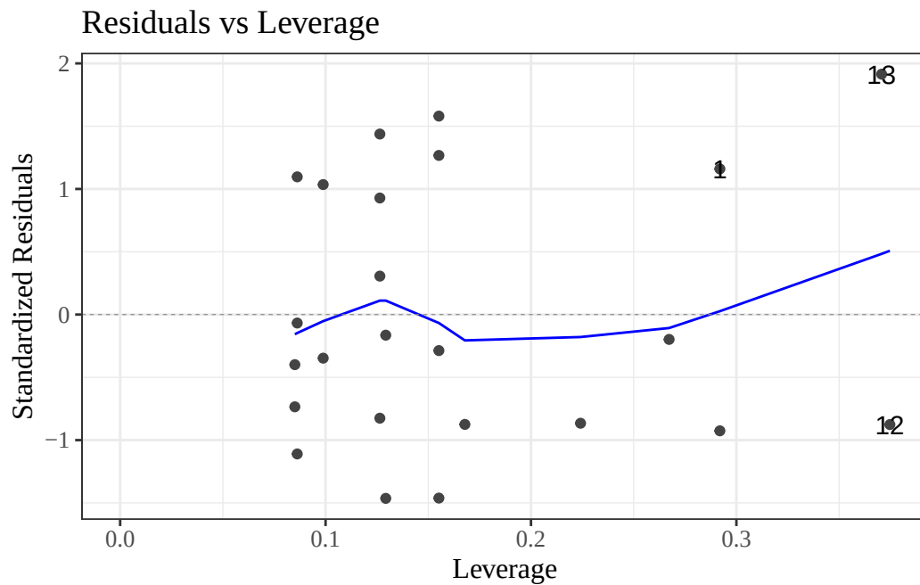
Figure 34: birthweight model with interactions (Equation 2): residuals versus leverage
