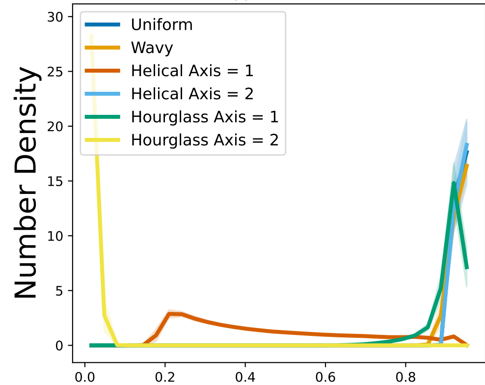
M_A = 0.25
