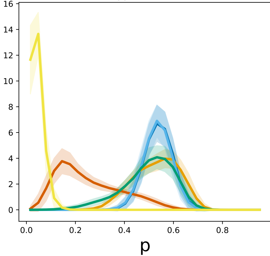
M_A = 0.75
