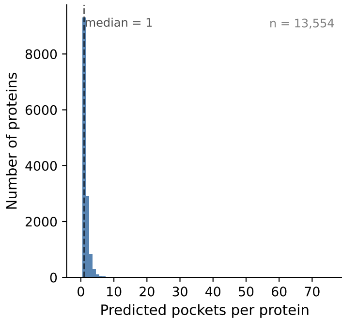
AF2Bind
