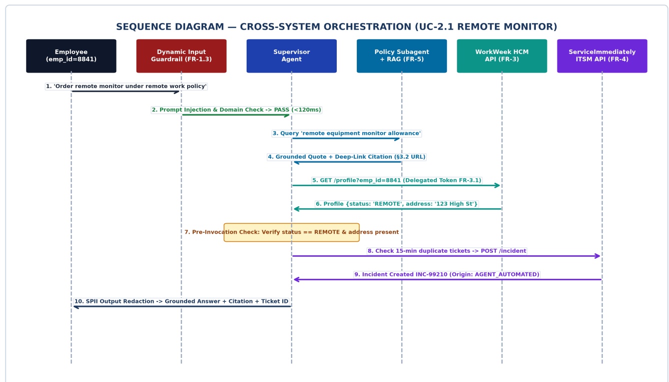
Figure 2: Multi-Turn Cross-System Orchestration Sequence Diagram (UC-2.1 Remote Hardware Order)
