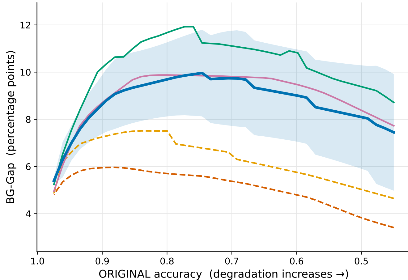
BG-Gap vs Accuracy: Positional vs Control Degradations
