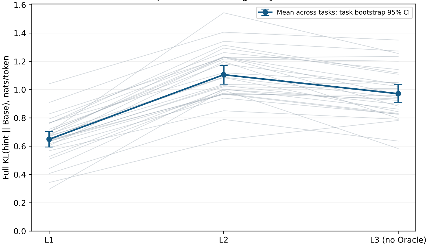
Same Base prefixes: reasoning body, 30 tasks, T=1
