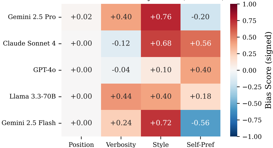
Baseline Bias Scores by Model (B0 Naive)
