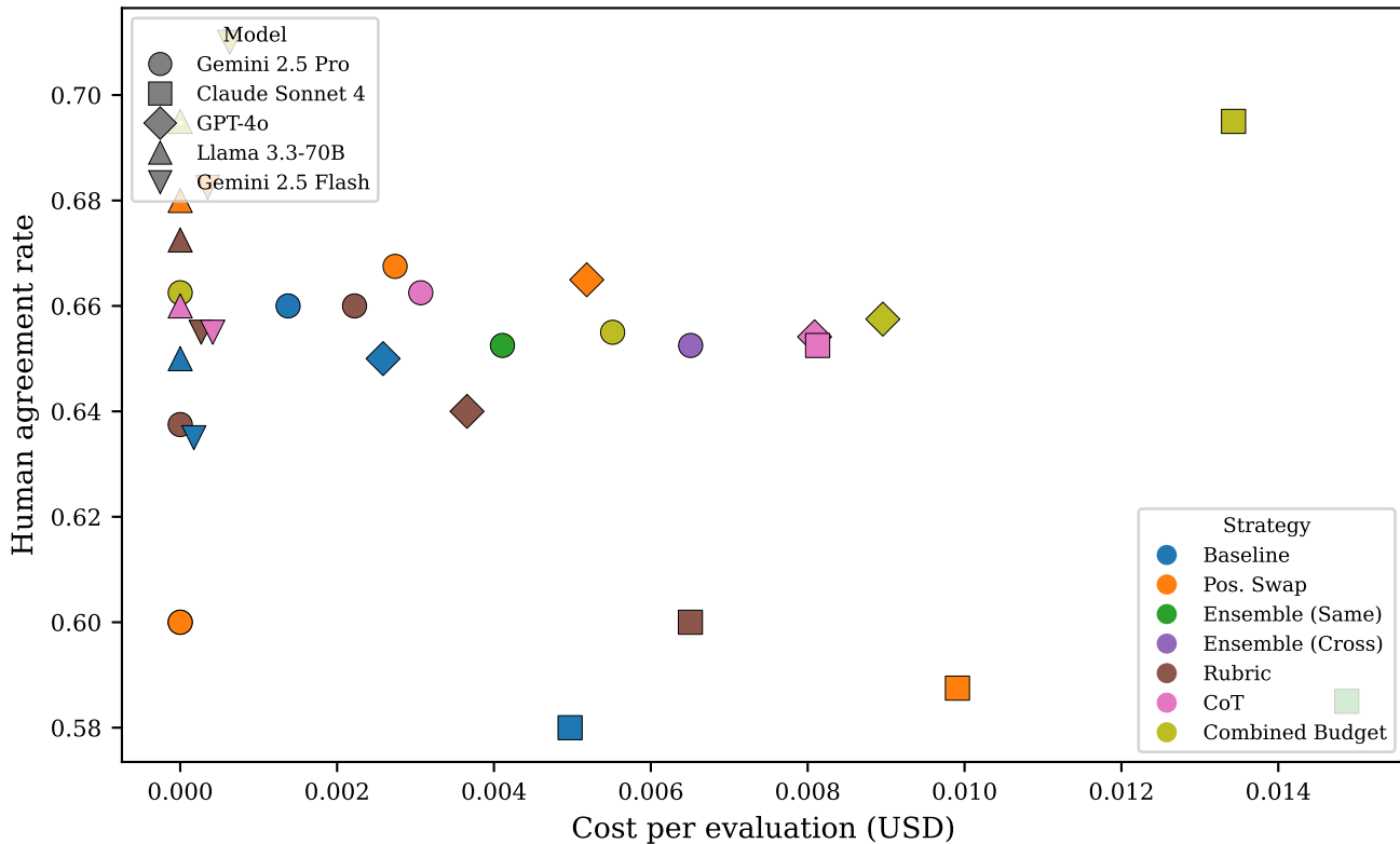
Cost vs Accuracy Tradeoff (MT-Bench)
